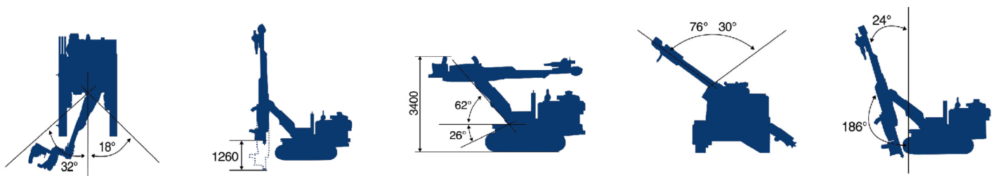
1. Swing angle of drill arm 2. Carriage compensation 3. Drill arm pitch angle 4. Sliding angle of the carriage 5. Carriage pitch angle
