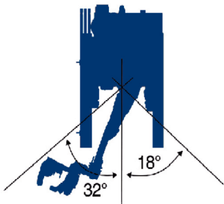
1. Swing angle of drill arm
