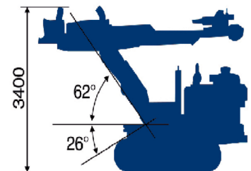
3. Drill arm pitch angle
